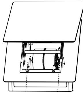
Aluminum Cassette Filter
